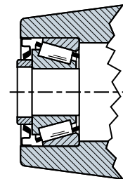
Sealed bearing configuration
