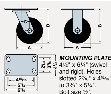
#S-628-UYB Swivel showing Unilast® Solid Elastomer wheel
