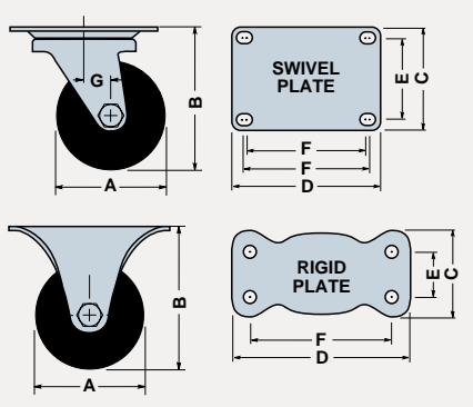
#S-224-EO Swivel showing Ebonite wheel
