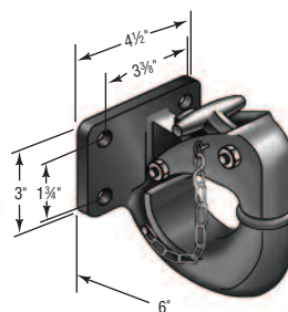
CP00120 Pintle Hitch Wt. 7½ lbs.
