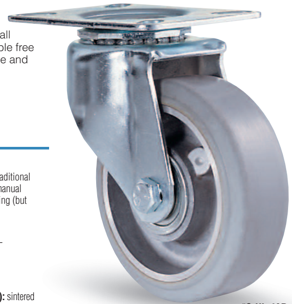
#S-HL-4AR Swivel showing Vulcalite™ wheel
